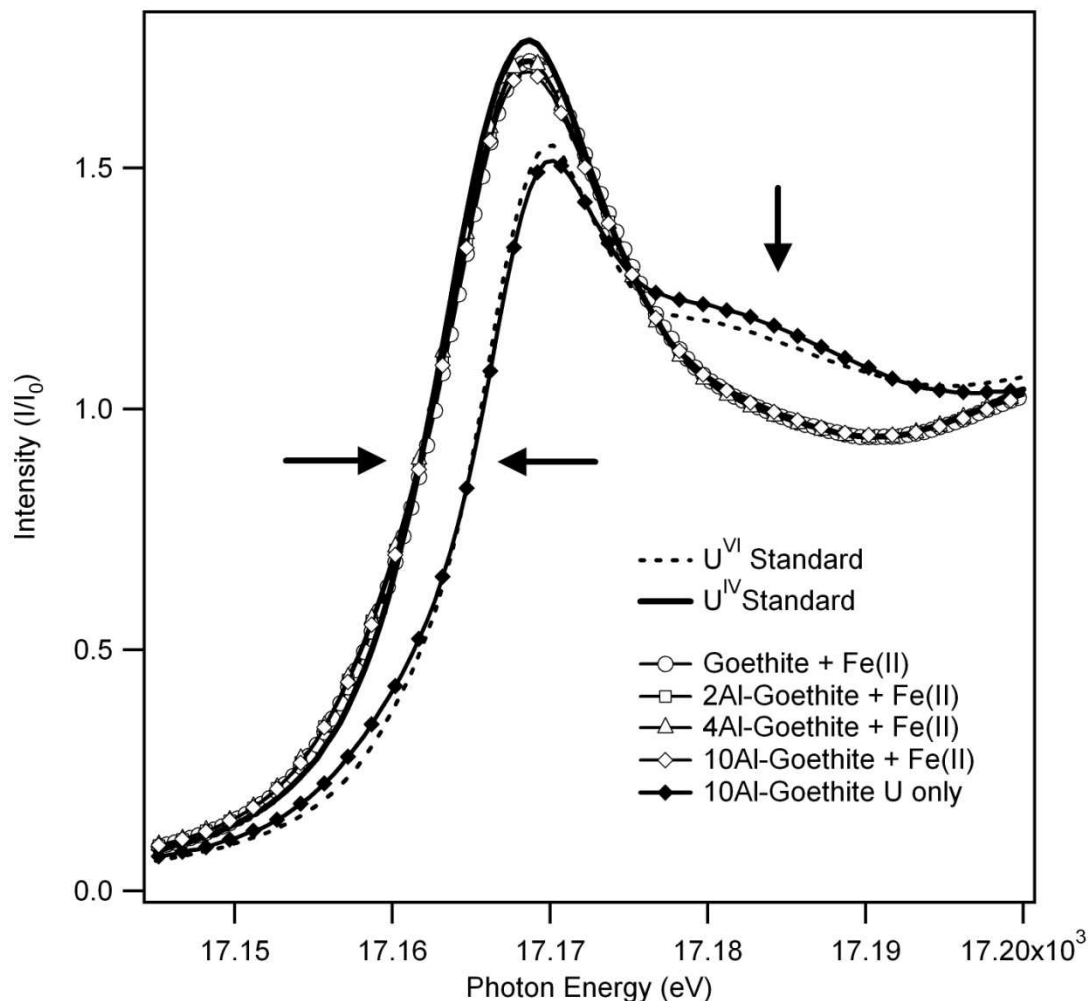
Figure 6.4. Uranium L_3 XANES spectra of U^{VI} reacted with goethite and Al-goethite in the presence of Fe(II). The horizontal arrows highlight the edge position, which is sensitive to U valence state with U^{IV} to the left and U^{VI} to the right. The vertical arrow points out the higher intensity post-edge feature for U^{VI} indicative of U in the uranyl ( UO_2^{2+} ) geometry. In all cases where Fe(II) is present U^{VI} is reduced to U^{IV} . U^{VI} remains in the 10Al-goethite sample without Fe(II).
